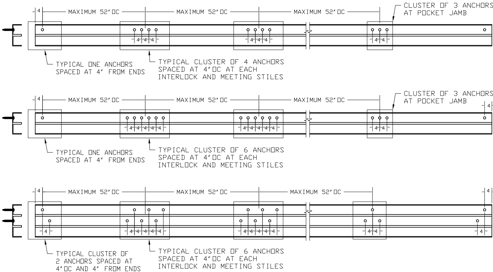
2 TRACK SYSTEMS ANCHORS TYPE A OR D
