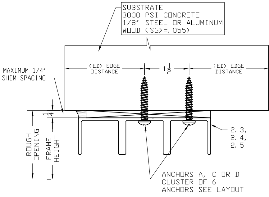
2 TRACK SYSTEMS ANCHORS TYPE A OR D
